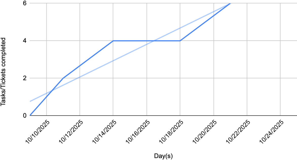
Burnup Chart
